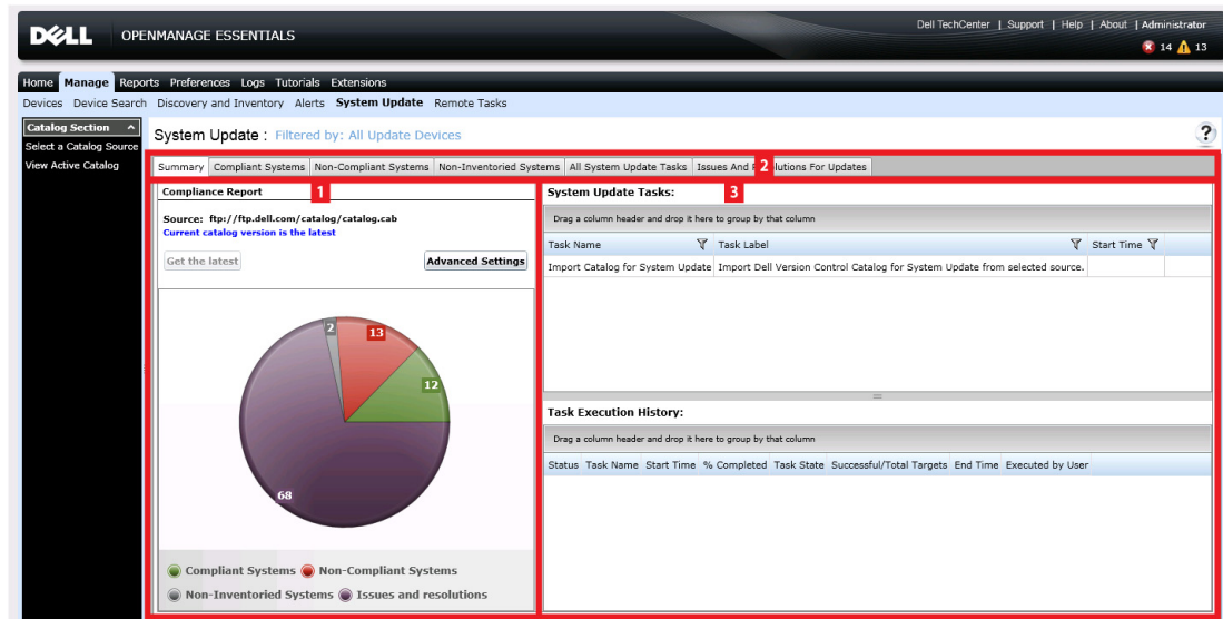
Figure 6. System Update Page
